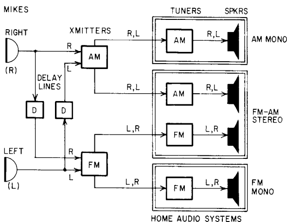
Fig. 619. Similar to the Bell simulcasting system, the Becker method also utilizes time delay circuitry and can be used in several combinations of transmitting media, including FM multiplex.
