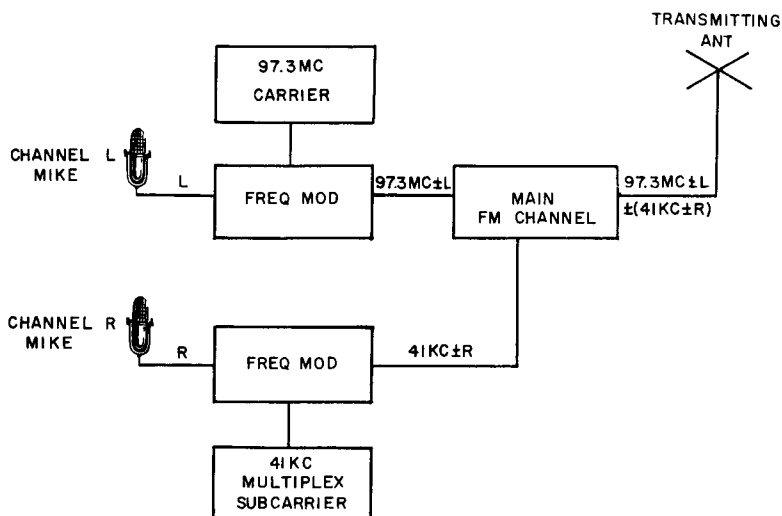
Fig. 608. In FM multiplexing, a principal channel is carried conventionally by the carrier, while a second channel modulates a subcarrier of 41 kc. The modulated subcarrier in turn modulates the main rf carrier.
