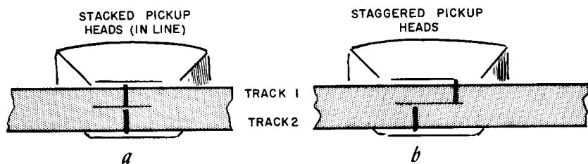
Fig. 401. (a) Stacked and (b) staggered stereo pickup heads. The staggered arrangement was used to facilitate conversion of mono tape recorders to stereo playback, but improved equipment and methods have made this system unpopular. Staggered tapes are no longer being manufactured.
