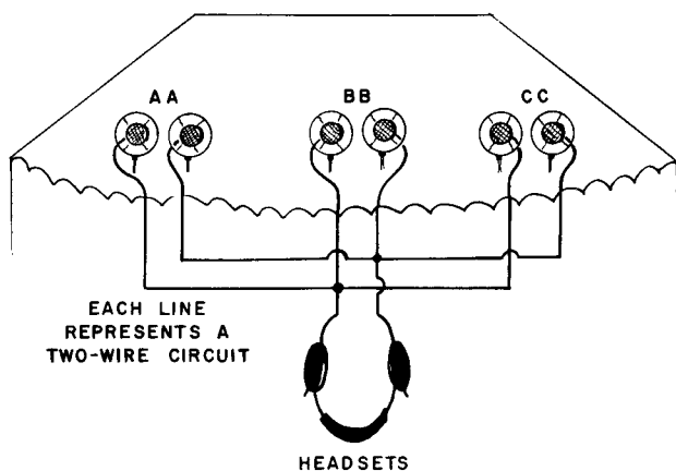
Fig. 202. Diagram of the stereophonic pickup system used at the Berlin Opera House in 1925.
