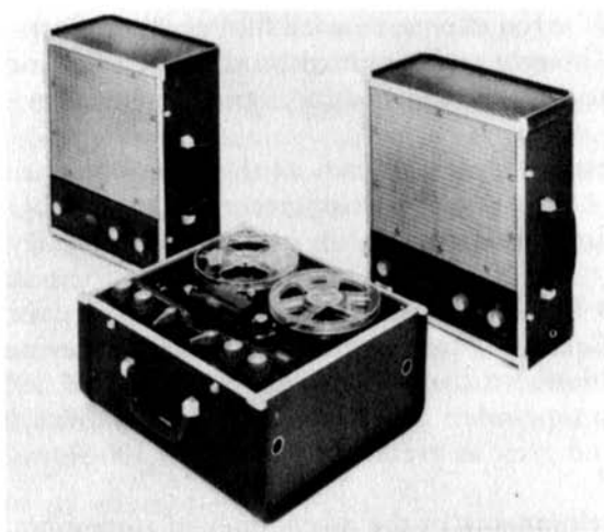
Fig. 404. A complete stereo tape system can come in a small package. Separate amplifiers are mounted in the two speaker cabinets. (Ampex)
