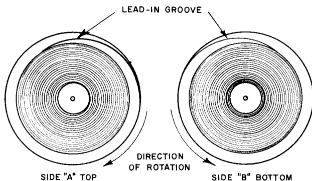
Fig. 502. Stereo recording on opposite sides of the disc.
