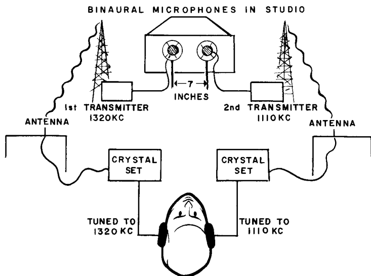
Fig. 203. The binaural broadcasting method of station WPAJ in 1925.
