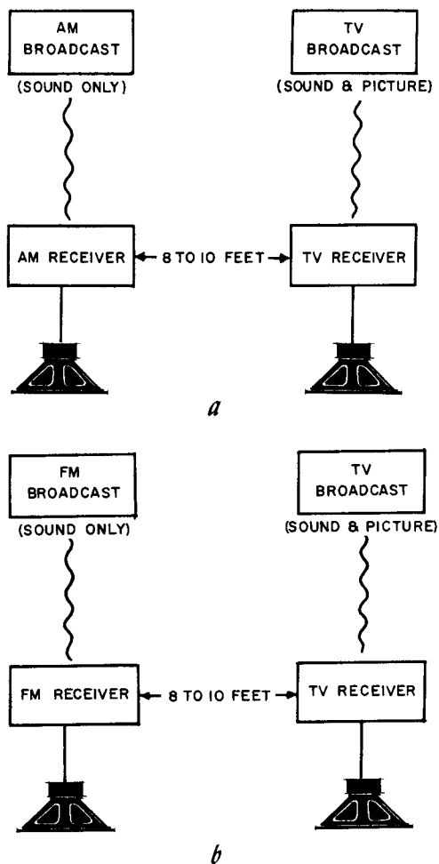
Fig. 605. Other methods of simulcasting use a television-station sound system for the right channel while an AM or FM station broadcasts the left.
