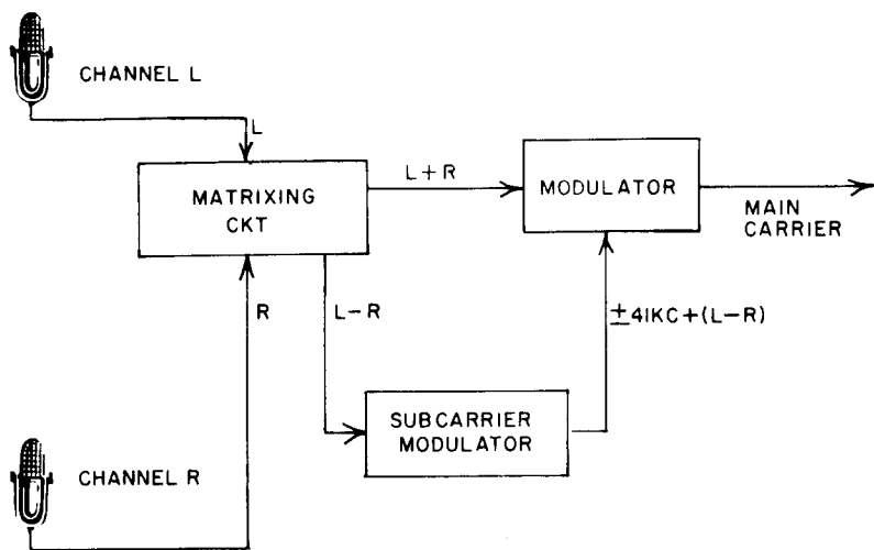
Fig. 615. Block diagram of Crosby method of modulation.
