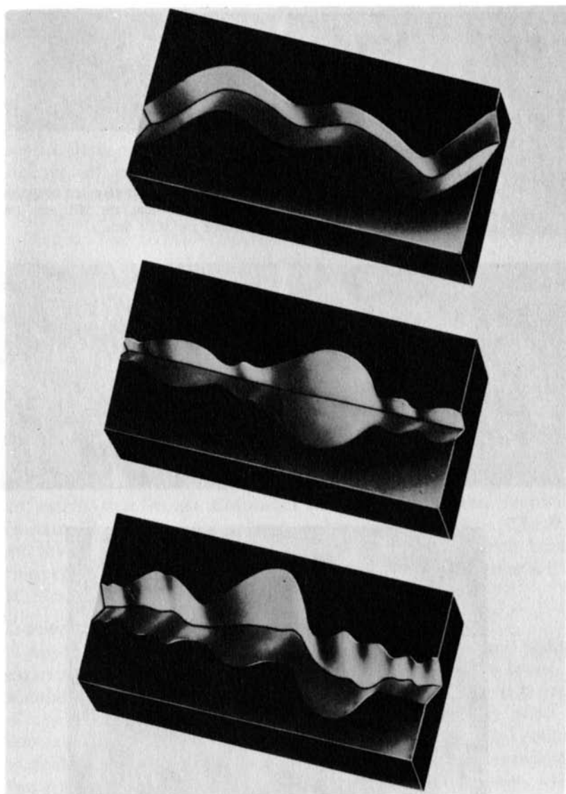
Fig. 505. Record groove modulation; (a) lateral cut, (b) vertical cut and (c) vertical-lateral combined in a stereo disc. (Telefunken G. M. B. H.)
