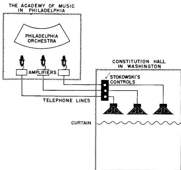
Fig. 211. Simplified diagram of the Bell Telephone Laboratories three-channel "broadcast".
