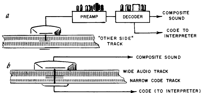
Fig. 403. Coded stereo can be reproduced by using a single coded track (a) or a wide audio track and an accompanying narrow code track (b).
