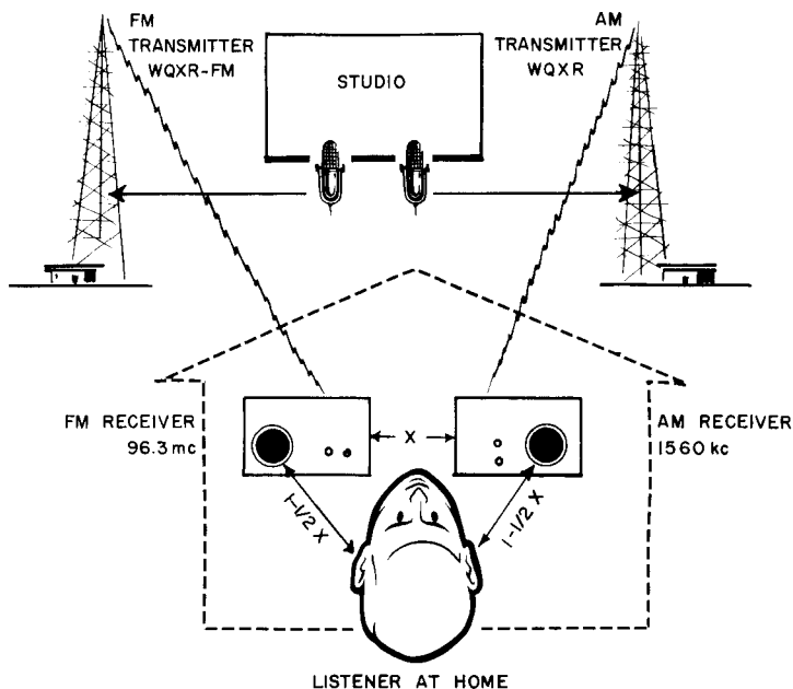
Fig. 601. AM-FM stereocasting system used by stations WQXR and WQXR-FM in New York City. The FM channel carries the left-channel signal, while the right channel goes out via AM.
