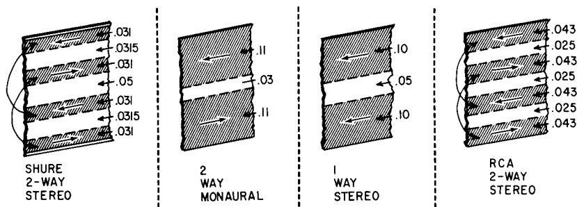
Fig. 410. Diagrammatic comparison of monophonic and two-track stereo tapes with the four-track system which was not adopted by the industry, and the RCA system, which was.
