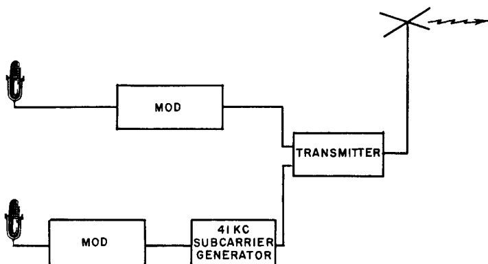
Fig. 609. Schematic diagram of the multiplex method used in musicasting. The subcarrier signal is added at the transmitter.
