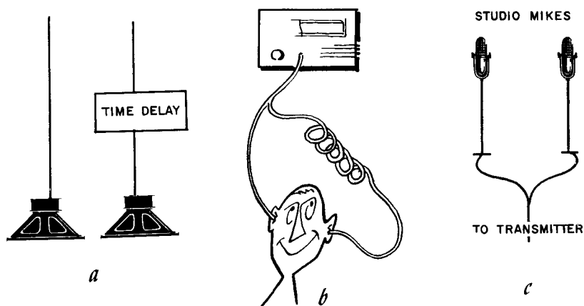
Fig. 702. Three early suggestions for achieving a pseudo-stereo effect from a monophonic source.
