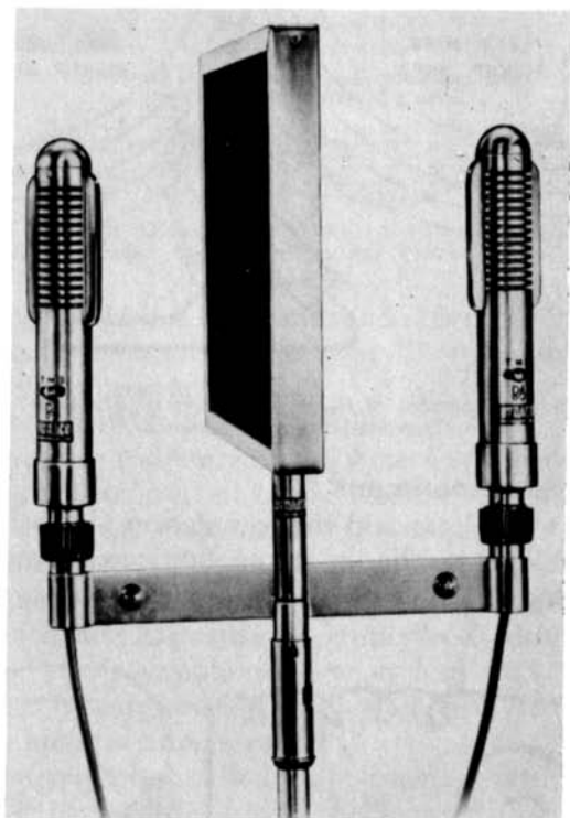
Fig. 208. This arrangement of microphones is still sometimes used today, with a baffle to simulate the acoustic effect of the human head. However, the figure-eight pickup pattern of these special microphones results in an apparent separation of as much as 10 feet. (Dynaco, Inc.)
