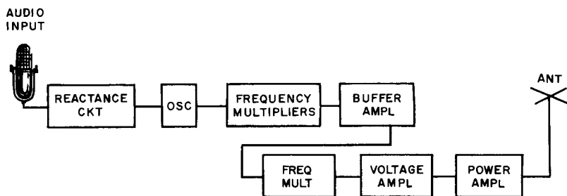
Fig. 610. Block diagram of FM transmitter used in commercial broadcasting.
