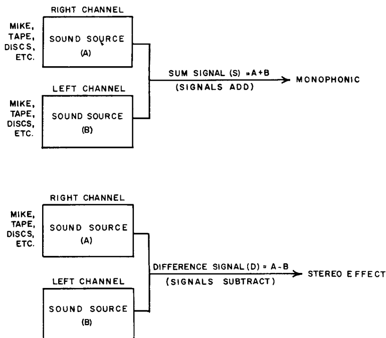
Fig. 612. Monophonic and stereophonic reception of a matrixed stereo-cast by multiplex.
