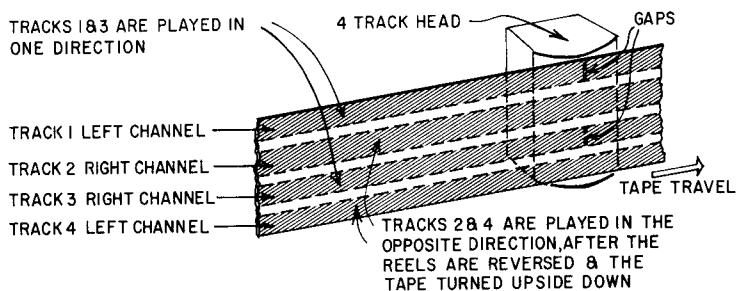
Fig. 409. Four-track stereo tapes have become the industry's standard because of their doubled playing time. The actual arrangement of the four tracks is shown here.
