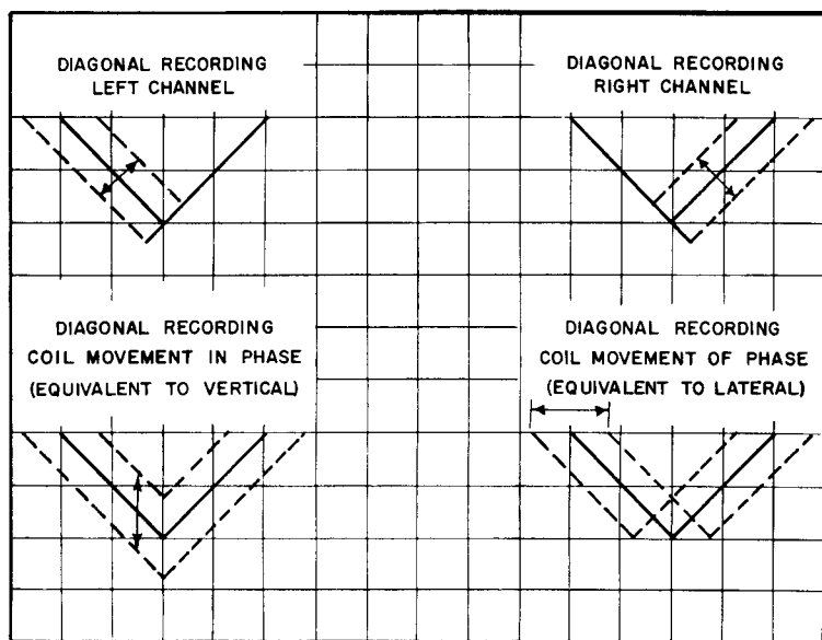
Fig. 508. (a) Comparison between laterally-cut groove (monophonic) and 45/45 stereo groove. (b) Stylus motion in stereo recording. (Westrex Corp.)
