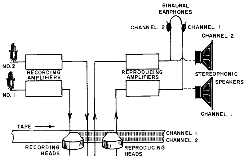
Fig. 402. A two-track stereo tape recorder using stacked recording and pickup heads. The stacked heads are shown as single units in this simplified diagram.
