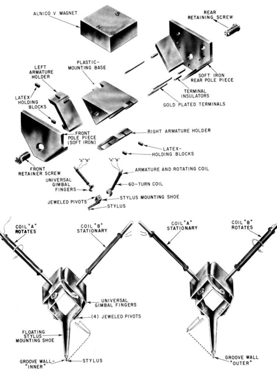
Fig. 509. (Top) Exploded view of magnetic stereo cartridge shows how the two independent rotating coils move in the field of a single Alnico magnet. Lower drawings show magnified detail of the stylus mounting and coil assemblies. Gimbal fingers allow maximum rotation in all directions resulting in high compliance.
