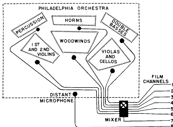
Fig. 304. The stereophonic recording arrangement used for "Fantasia".
