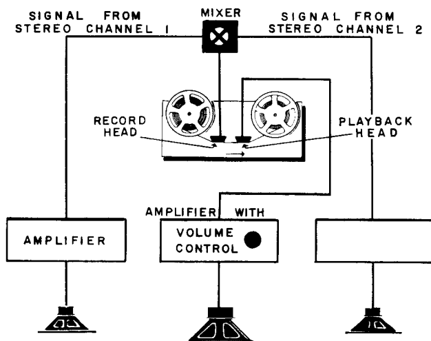
Fig. 307. The Bogert system, using time-delay to reduce the power requirements of the side channels in relation to the center channel.
