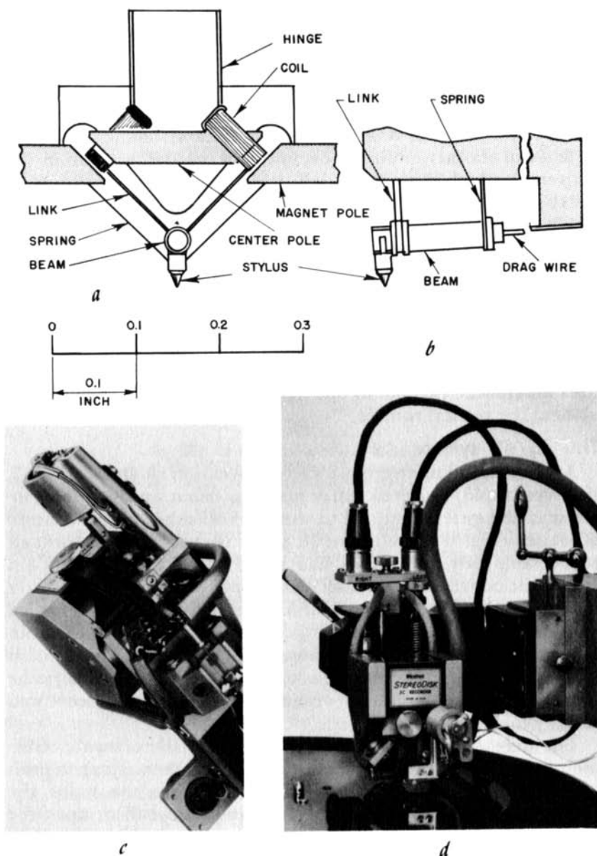
Fig. 504. (a) Cross-sectional view of the 45/45 cutting head. (b) Detail of the stylus mounting assembly. (c) Bottom view of the 3C cutter with automatic depth control. (d) 3C cutter mounted on a Scully lathe. (Westrex Corp.)
