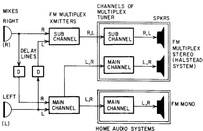
Fig. 620. Reception of stereocasts by the Becker method can utilize several possible combinations of broadcasting media including all-FM by multiplex, using the Halstead system.
