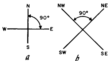
Fig. 503. Comparison of stylus motion in the "VL" (vertical-lateral) system (a) with stylus motion in the 45/45 system (b).
