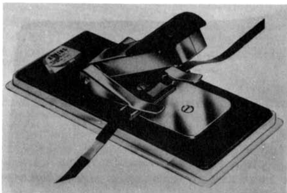
Fig. 408. A popular tape splicer which cuts slightly into finished splice for a "wasp-waist" effect. The splice made this way will pass smoothly and quietly over the tape heads. (Robins Industries, Inc.)
