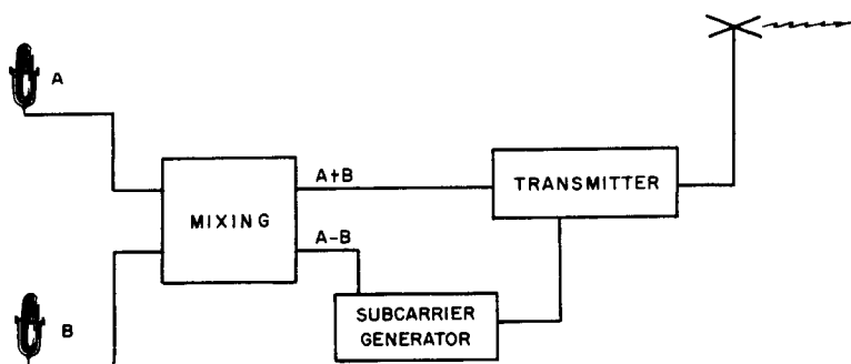
Fig. 613. The sum-and-difference method in transmission. The transmitter is modulated directly by both channels A and B, and also by a subcarrier generator modulated by frequencies which are the difference between the two audio channels.
