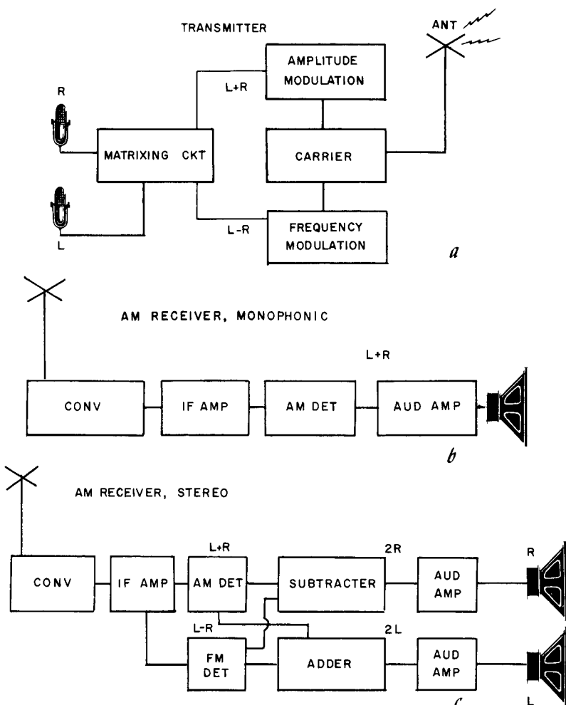
Fig. 618. The Westinghouse AM stereocasting system uses a matrixed signal similar to that of the Crosby system. The L + R signal amplitude-modulates the rf carrier in conventional fashion. The L - R signal frequency modulates the carrier (a). For monophonic reception (b), the L + R signal is conventionally received and detected by any AM radio. For stereo reception (c) a special receiver or an adapter attached to a conventional radio must be used.
