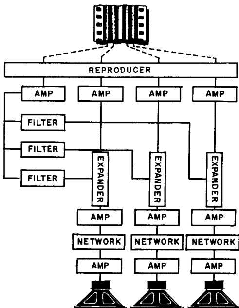
Fig. 303. Schematic diagram of the stereophonic reproducing circuits. (Journal of the SMPE.)
