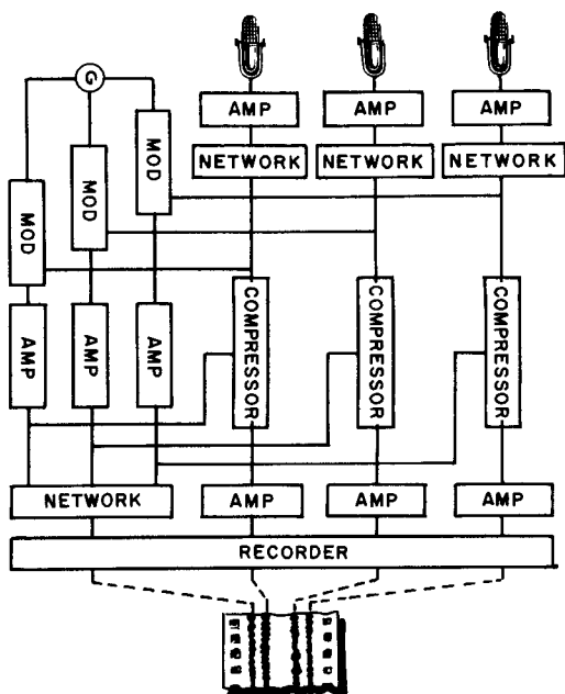
Fig. 302. Schematic diagram of stereophonic recording circuits. (Journal of the SMPE.)
