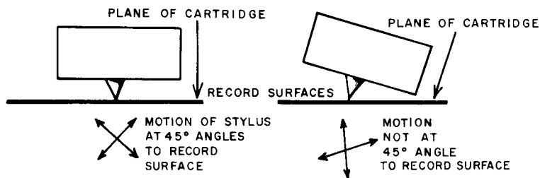
Fig. 507. Crosstalk can be due to misalignment of stereo pickup.
