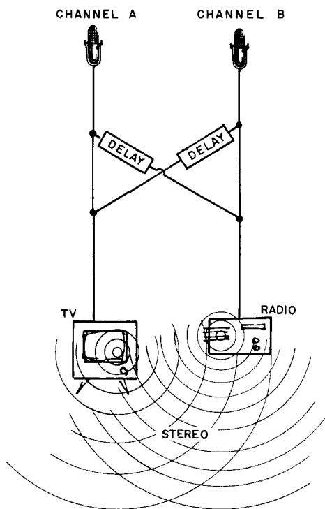
Fig. 617. Bell Laboratories stereocasting system which may be used with any two broadcasting mediums, and is compatible.
