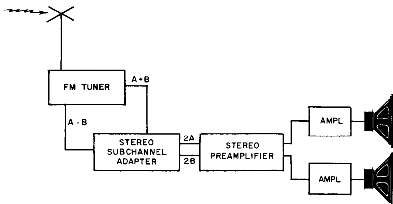
Fig. 614. In the reception of the matrixed stereo signals, the main carrier and subcarrier are separated at the discriminator and fed to adder and subtractor circuits. The resulting 2A and 2B signals then go to the stereo preamp and amplifiers.
